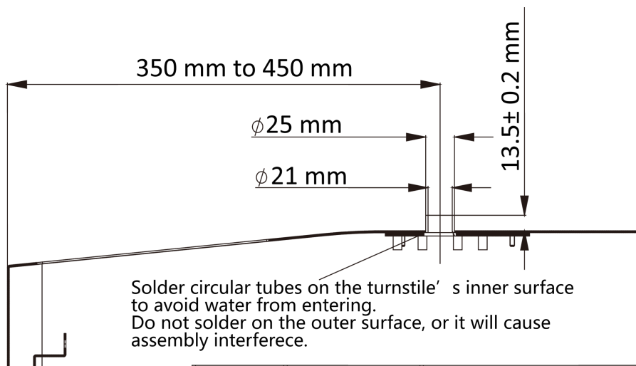
Figure 3-2 Solder Tubes
