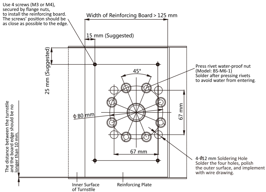
Figure 3-1 Drill Holes on Turnstile
