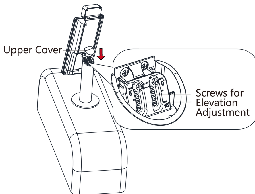
Figure 3-5 Adjust Elevation
