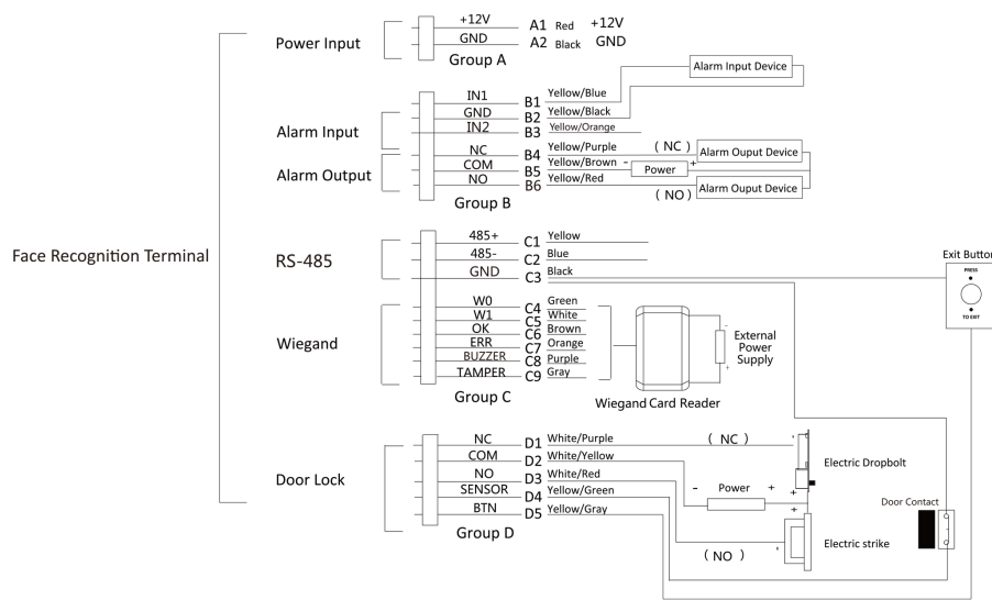
Figure 4-2 Device Wiring
