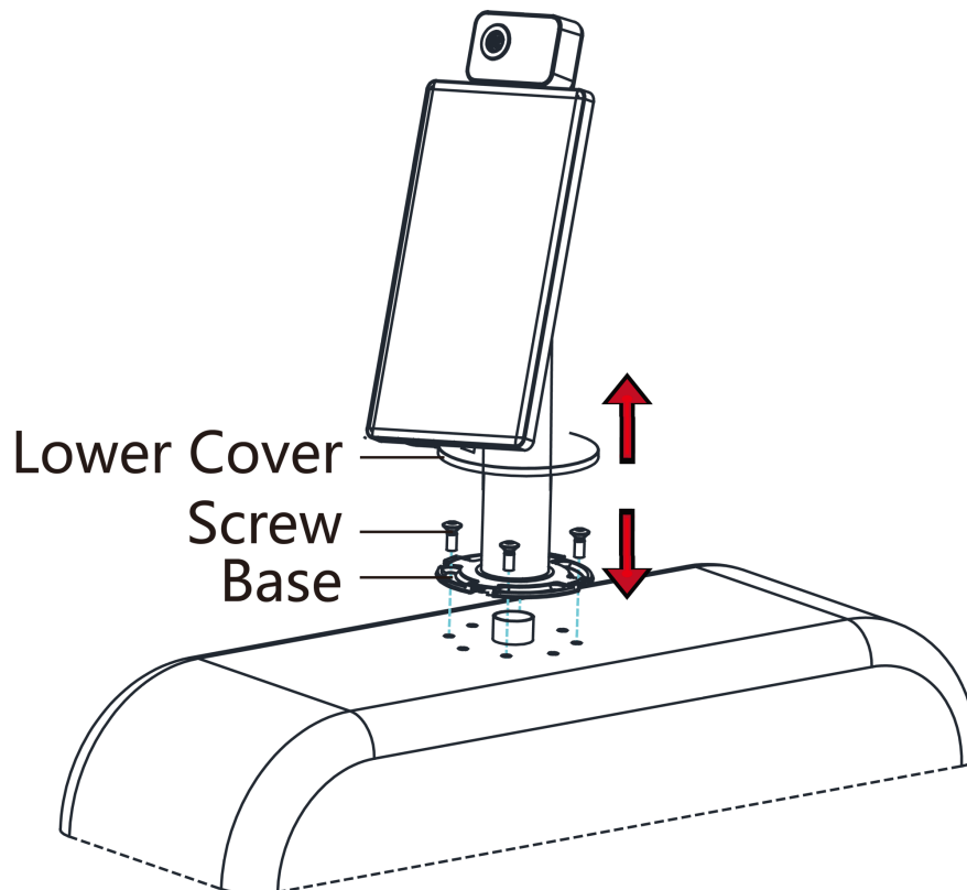
Figure 3-3 Secure Bracket and Turnstile
